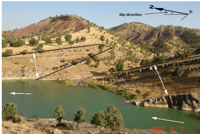
Figure 5: Northwest dipping lateral thrust on the Aqra Formation (or Lens) at 2km south of Kele village, on the right bank of Dolbeshk stream. The limestone succession (A) is repeated by thrusting which is about 20m thick. The longitude and latitude reading of GPS of this location is (N: 35 48 17.55 and E: 45 26 99).
