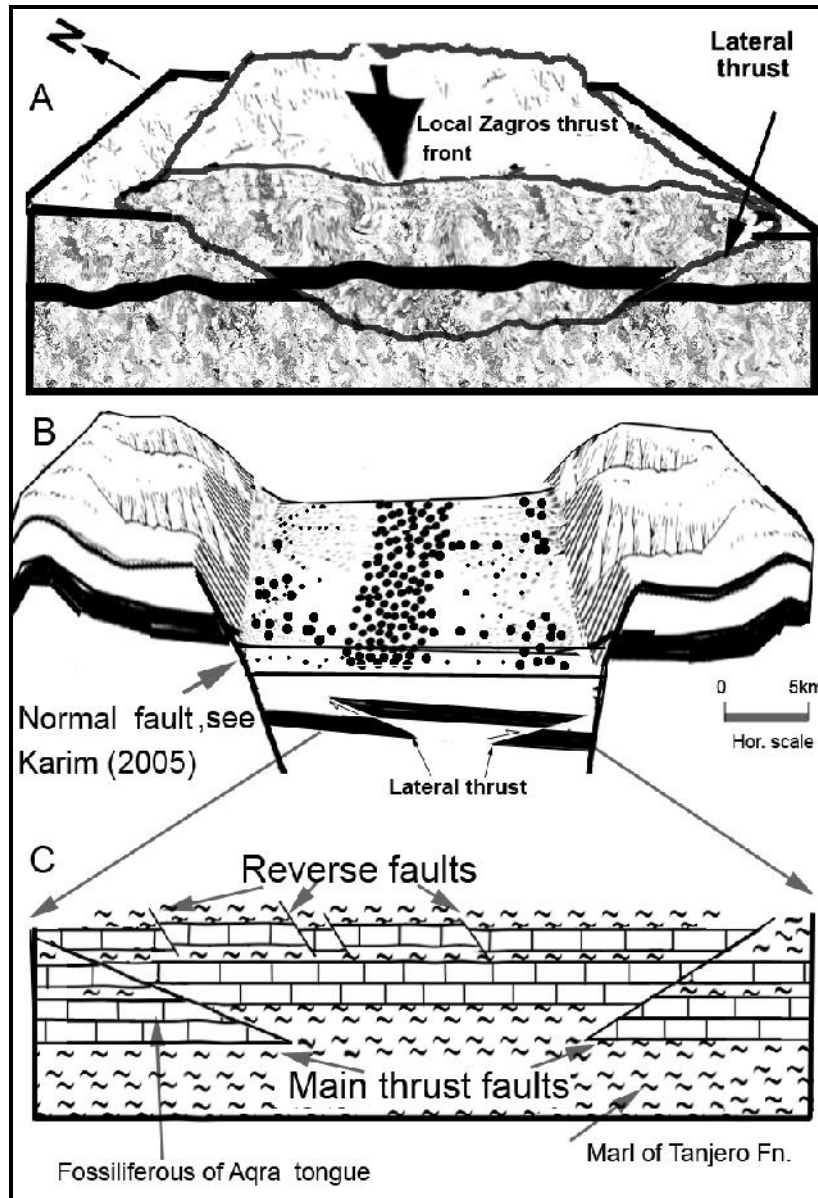
Figure 8: Field based sketches to show the possible origins of both the large lateral thrust faults and a small reverse faults. A) Lateral thrusts as a boundary of the local front of Main Zagros Thrust
