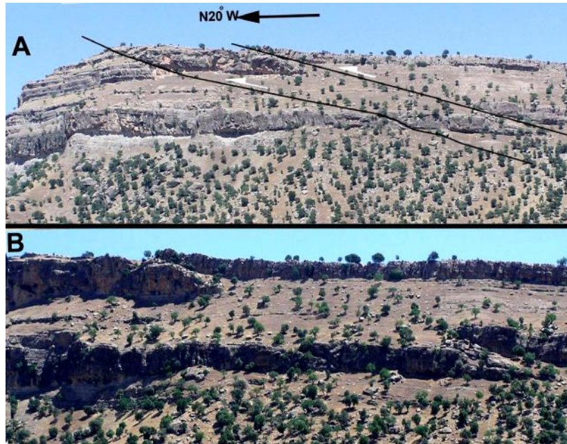
Figure 2: A) an erosional scarp at northeast of Kareza village showing southeast dipping lateral thrust cutting two limestone beds of the Aqra Formation, each about 7m thick at station five (St5). B) Close up view of the upper fault.
