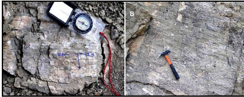
Figure 4: A and B) fault surface showing striation and mineralization. These features exist only on the surface of small reverse faults between the lateral faults. Both the compass and hammer are pointing toward north. The Hammer head is pointing to north.
