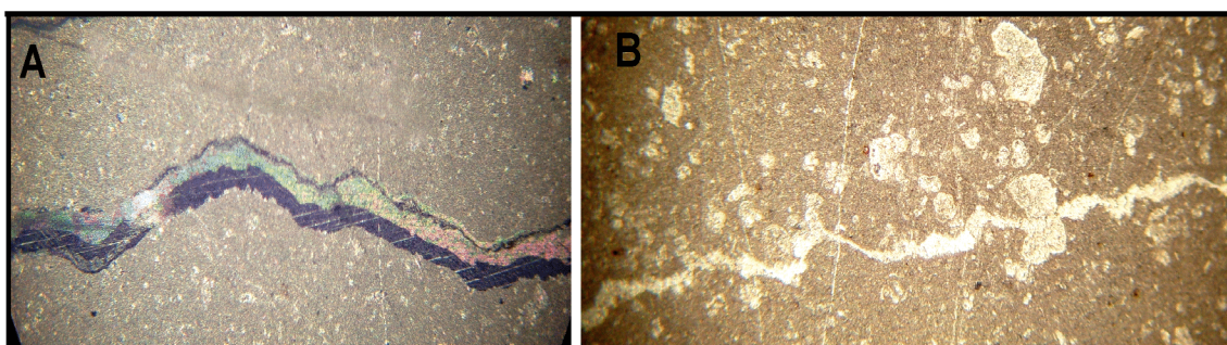
Fig.5: Crenulations under polarized microscope (40 X), showing microscopically folded fractures. A) Under XP light shows two phases (dark and light) band of filling of fracture with secondary spary calcite. B) Under normal light shows a folded fracture, which cut across a Globotruncana foram
