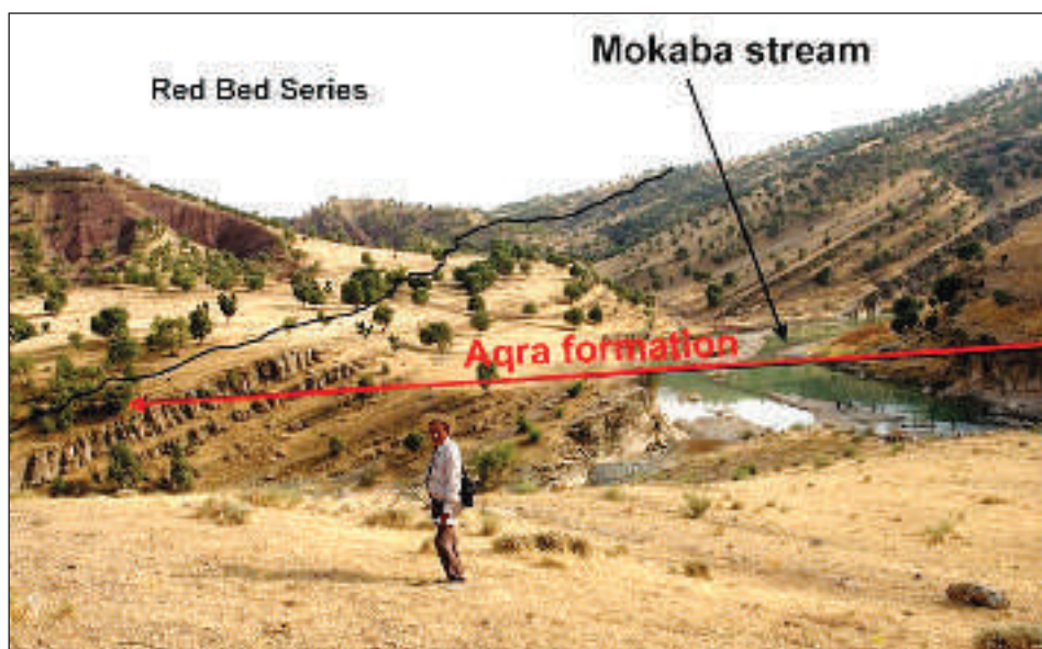
Figure 4- Khewata section showing the relationship of the Aqra Formation with Red Bed Series in the northern boundary of the studied area, looking southeast.
