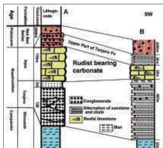
Figure 3- Stratigraphic columns showing the setting of the Aqra Formation in the succession at Mawa-Chuerta area (after Karim et al., 2007). A. The column for the northern boundary of the studied area (Khewata section). B. The column for the southern boundary of the studied area reflecting Suraqalat and Sherawazha sections.
