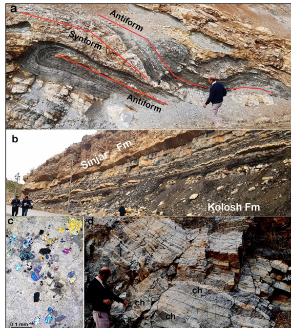
Figure 11. a) Intensive deformation limb-on-limb antiforms and a synforms (bended 180 degrees and overturned toward southwest, the red lines are traces of axial plain of folds. It is regionally metamorphosed volcanoclastic sandstone (greywacke) overlain by marble (limestone) without contact metamorphism. They were considered previously as layered gabbro, a section along the road cut at latitude and longitude of 36° 9' 55.18" N and 45° 15' 9.64" E on the paved road to Kele Border Check point. b) If the succession in the photo (a) is restored to a horizontal condition before deformation, it would look exactly like the contact between Kolosh and Sinjar Formations as appears from the photos (b) at 500 m southwest of Kalk Smaq village Dokan area. The rocks of both photos nearly have the same ages (Paleocene-Eocene). c) Calc-silicate rock with olivine (colored grains) and calcite (grey) near the Iranian border on the paved road on the top of the Bulfat Mountain, s.no.11, XPL. d) The alternation of the felsic and mafic-rich layers of volcanoclastic sandstones with small channels (ch) at 300 m west of Beklo village. These rocks were previously considered as gabbro and diorite.
