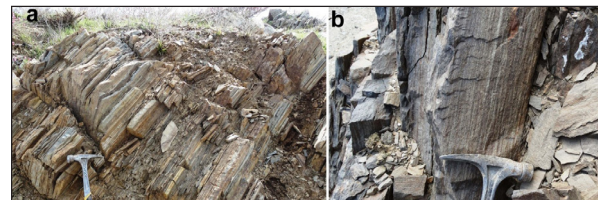
Figure 4. Metamorphosed volcanoclastic greywackes and shale. a). preserved original bedding. b). preserved millimetric sedimentation laminae on the head of Shilana Valley 300 m to the north of police check point at latitude and longitude of 36° 11' 32.89" N and 45° 17' 00.86" E.
