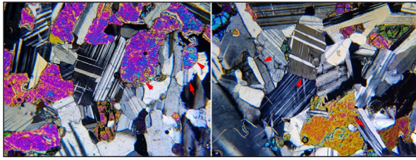
Figure 16. coarse crystalline previous gabbro (present mafic granulite resulted from metamorphosed coarse-grain volcaniclasts sandstones which have sutures boundaries (red arrows) and no cumulate texture 500m to the west of the Iranian police station on the border on the Bulfat Mountain, s.no.12, XPL
