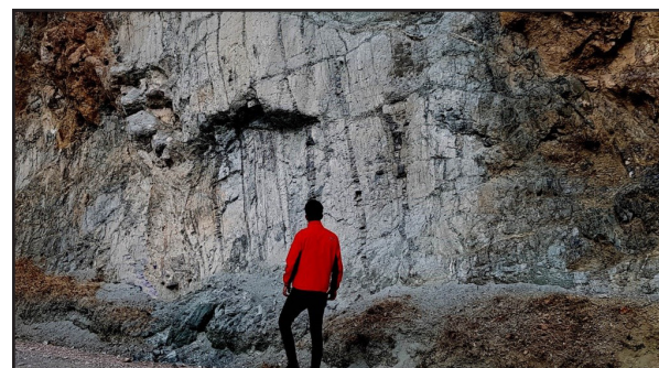
Figure 6. Same alternation at vertical attitude at latitude and longitude of 36° 9' 17.5 6" N and 45°14' 41.51" E, between Darashimana and Lower Beklo villages.
