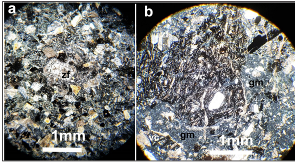
Figure 17. a). Volcaniclastic sandstone of Walsh-Naoperdan Series (in Mawat area) derived from volcanic source area and mostly consists of zoned plagioclase (zf) volcanic clasts under XP light, S.no. 15. b). The same sandstone shows large clast (grain) (vc) of volcanic rocks with fine-grained groundmass (gm).
