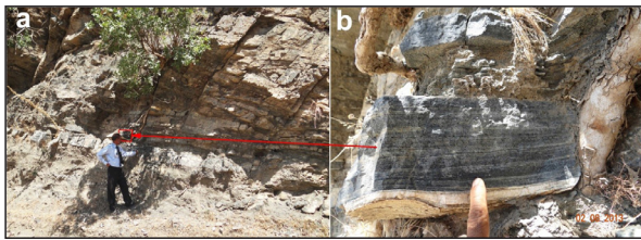
Figure 18. a). Metamorphosed succession of well-bedded and laminated volcaniclastic sandstone composed mainly of hornblende and plagioclase, exposed between the Beklo and the Wasena village at the latitude and longitude of 36° 9' 2.74" N and 45° 16' 0.32" E. b). A close-up photo of the laminated bed in the red circle shows regular and parallel laminations, the present study assumes that they are originally sedimentary and belong to the Walsh-Naoperdan Series.
