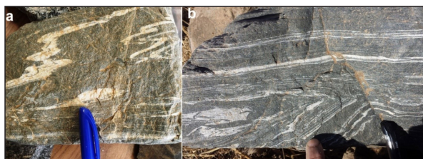
Figure 20. Intense deformation of the metamorphosed greywacke (with sedimentary felsic and mafic-grain-rich laminae), a) as ptygmatic folding of previous fractures, b) folding of white and black laminae in form of synforms and antiforms. These folds are deformed before metamorphism during tectonic burial.
