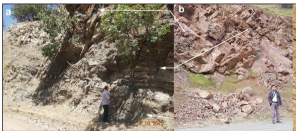
Figure 19. Comparison between: a). stacking pattern of the layered hornfels-like rocks (near the Beklo village) and b). Fresh the volcaniclastic sandstone (greywacke) of the Walsh-Naoperdan Series at 3km east of Mawat town on the road to the Gabara village.
